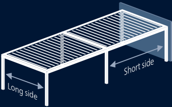
Coupling in transverse direction (constructions face to face on the wall) max. 24 metres
