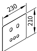
cover plate for spacer plates and stand-off brackets in the case of external insulation
