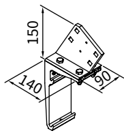
eaves fixture bracket
