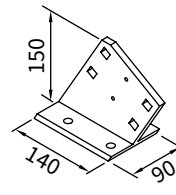
eaves fixture bracket
